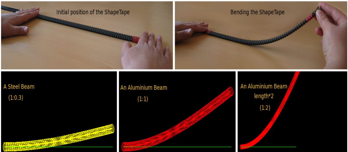
Fig. 3 A physically-based beam bending, controlled interactively by the ShapeTape. For the same tape displacement, the physical behavior of the beam changes according to the material (steel, aluminum) and
